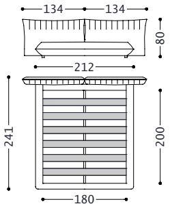
1BVLLA180B 1BVPLA180B
