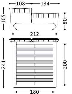
1BVLLA180AB 2BVPLA180AB
